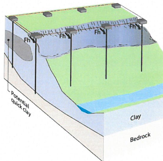
Figure 6 Scenario C - Damage to several piles in 1st row
