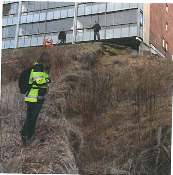
Figure 2 The backscarp of the slide. Vertical deformation 0,5-1 m.
