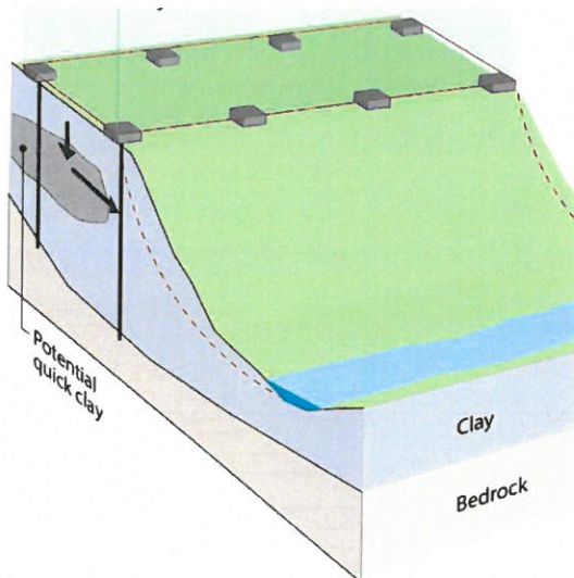
Figure 4 Scenario A - quick clay slide
