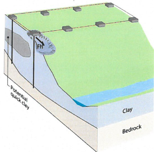
Figure 5 Scenario B - Damage to corner pile
